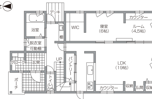
1F
