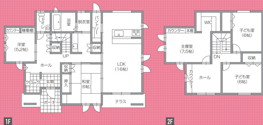
1F
